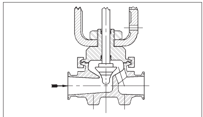
FIGURE 2 – Straight Body with Composition Plug
