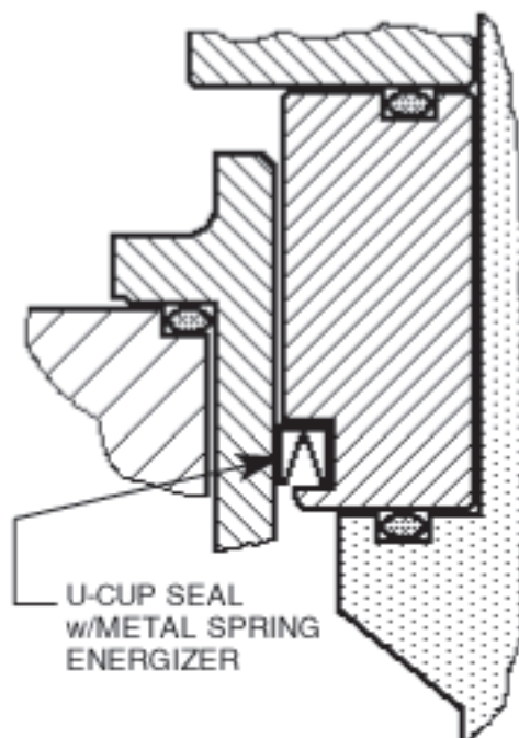
U-CUP DYNAMIC SEAL
