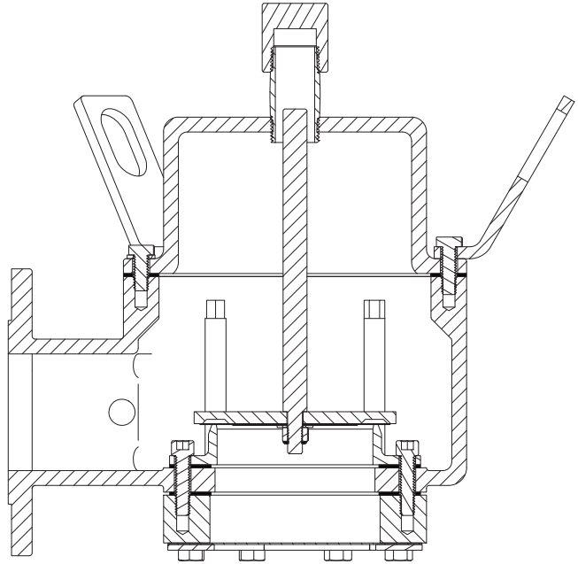
EXTENDED CONFIGURATION - SECTION VIEW
