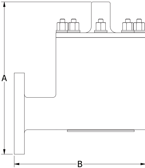
STANDARD CONFIGURATION - FRONT VIEW
