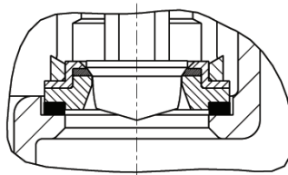
Figure 1 TFE-Soft Seat Design
